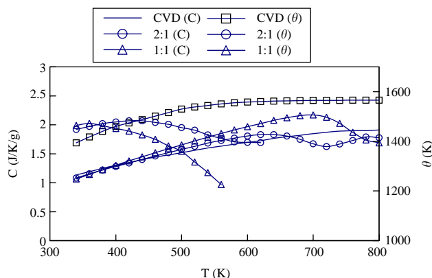
Fig. 3. Temperature dependence of heat capacity and Debye temperature. (The results of amorphous CVD wafer [3] are also shown.)
